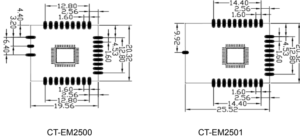
Figure 4 Mechanical Dimensions of CT-EM2500 and CT-EM2501 modules
